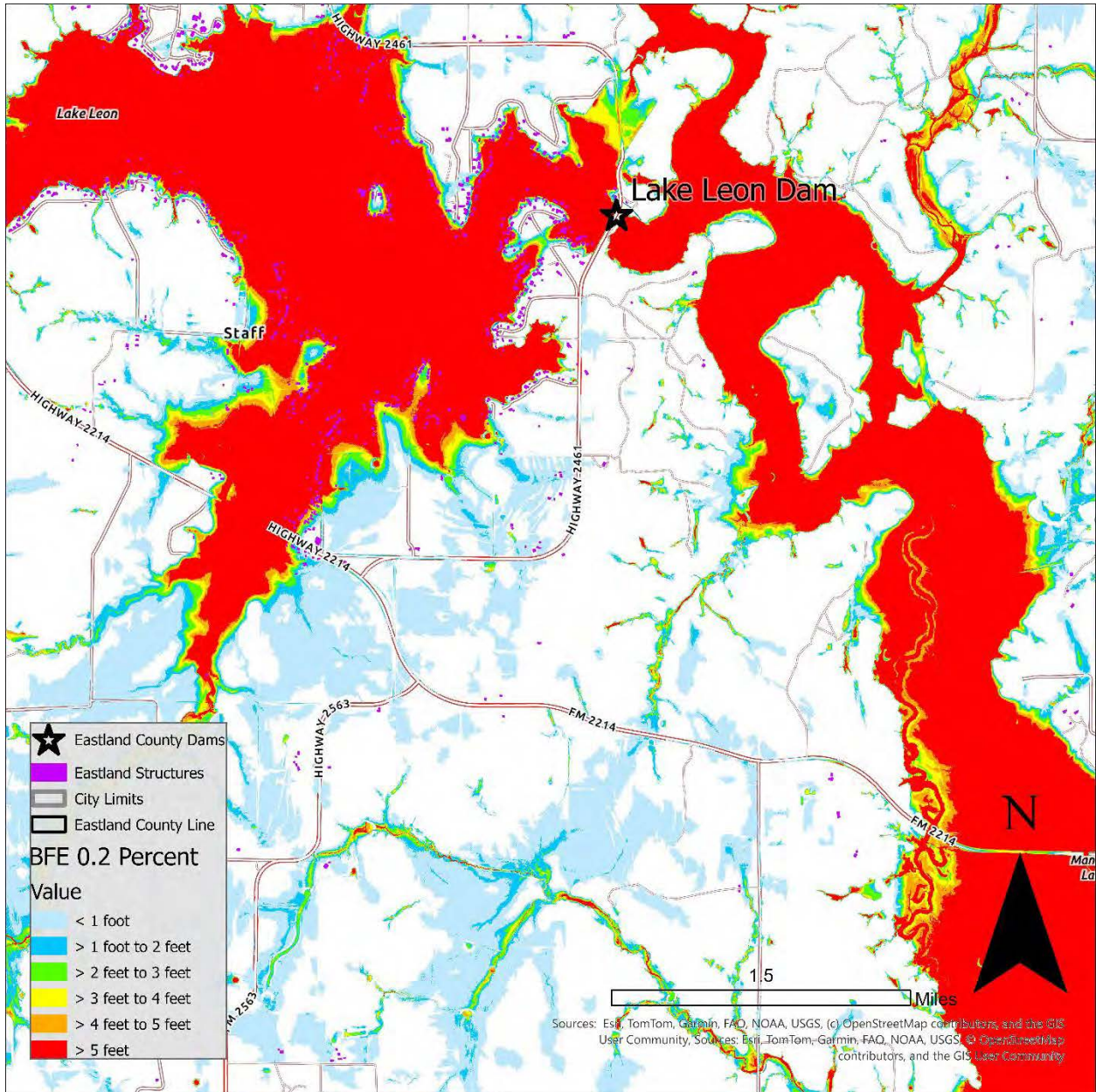
Figure 15-10: FEMA BFE surrounding Lake Leon Dam (Source: FEMA)
